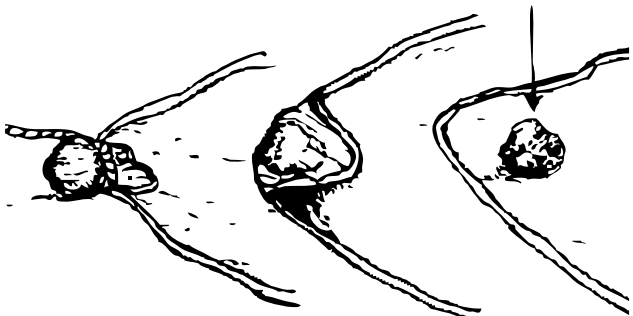
Bowline or Timber or Clove Hitch around rock
