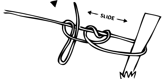
Taut-Line Hitch or Trucker's Hitch or Backhanded
